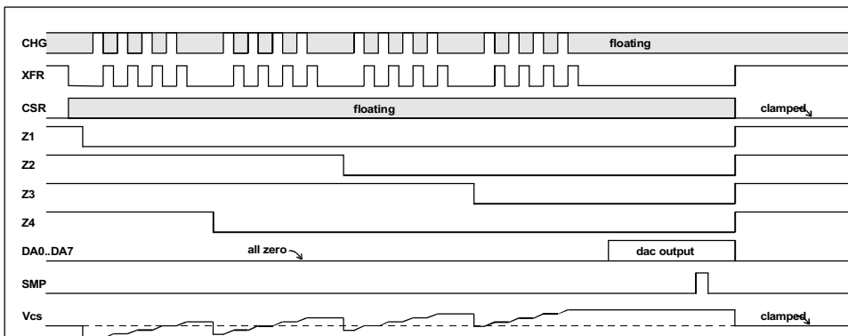
FIGURE 1-2 BURST WAVEFORMS
